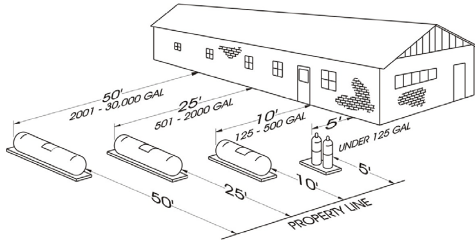
TYPICAL VIEW (SEE I.F.C. 3804 2003 EDITION SECTION 3804 FOR ADDITIONAL INFORMATION)
